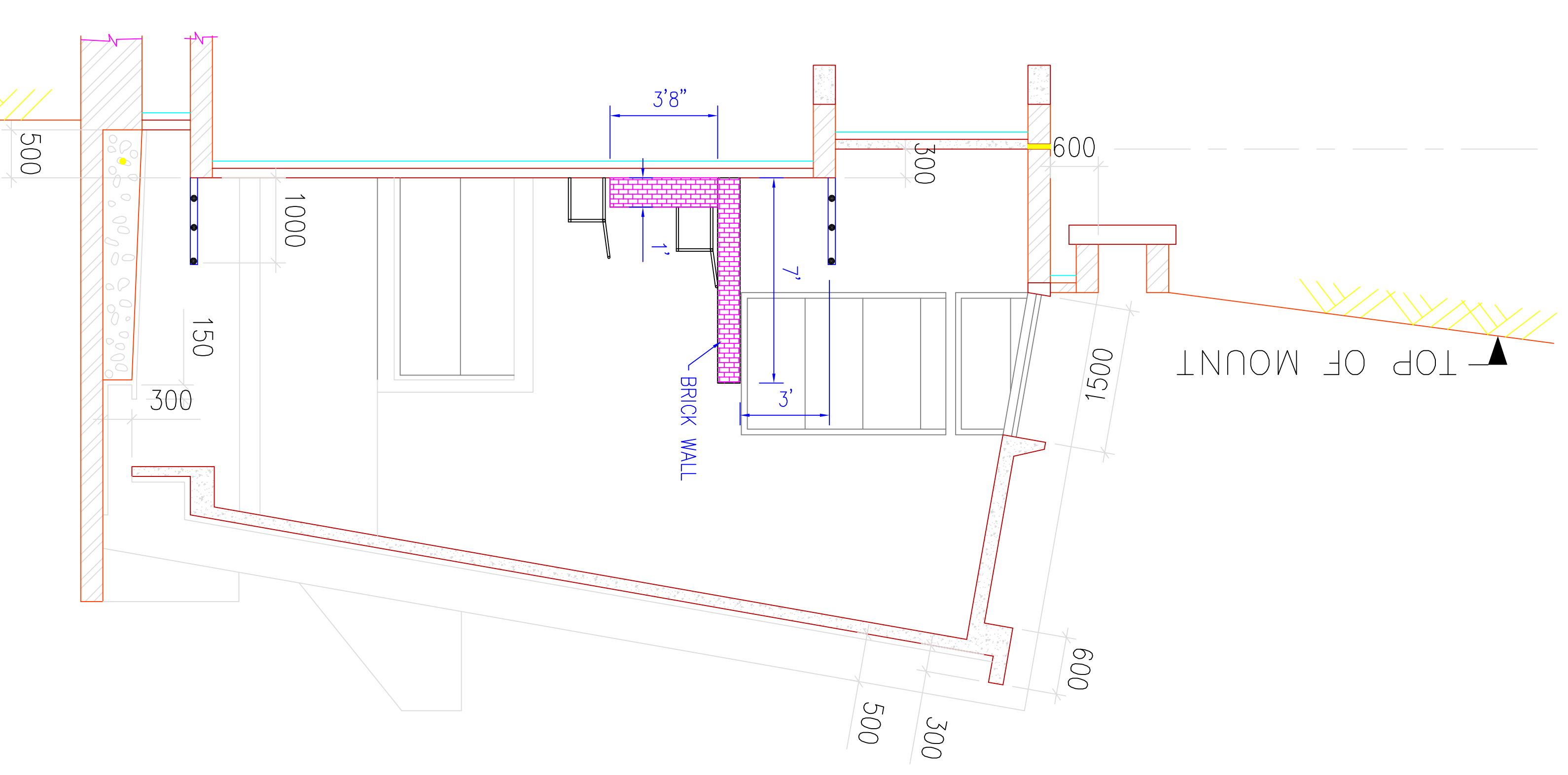
SECTION - AA
